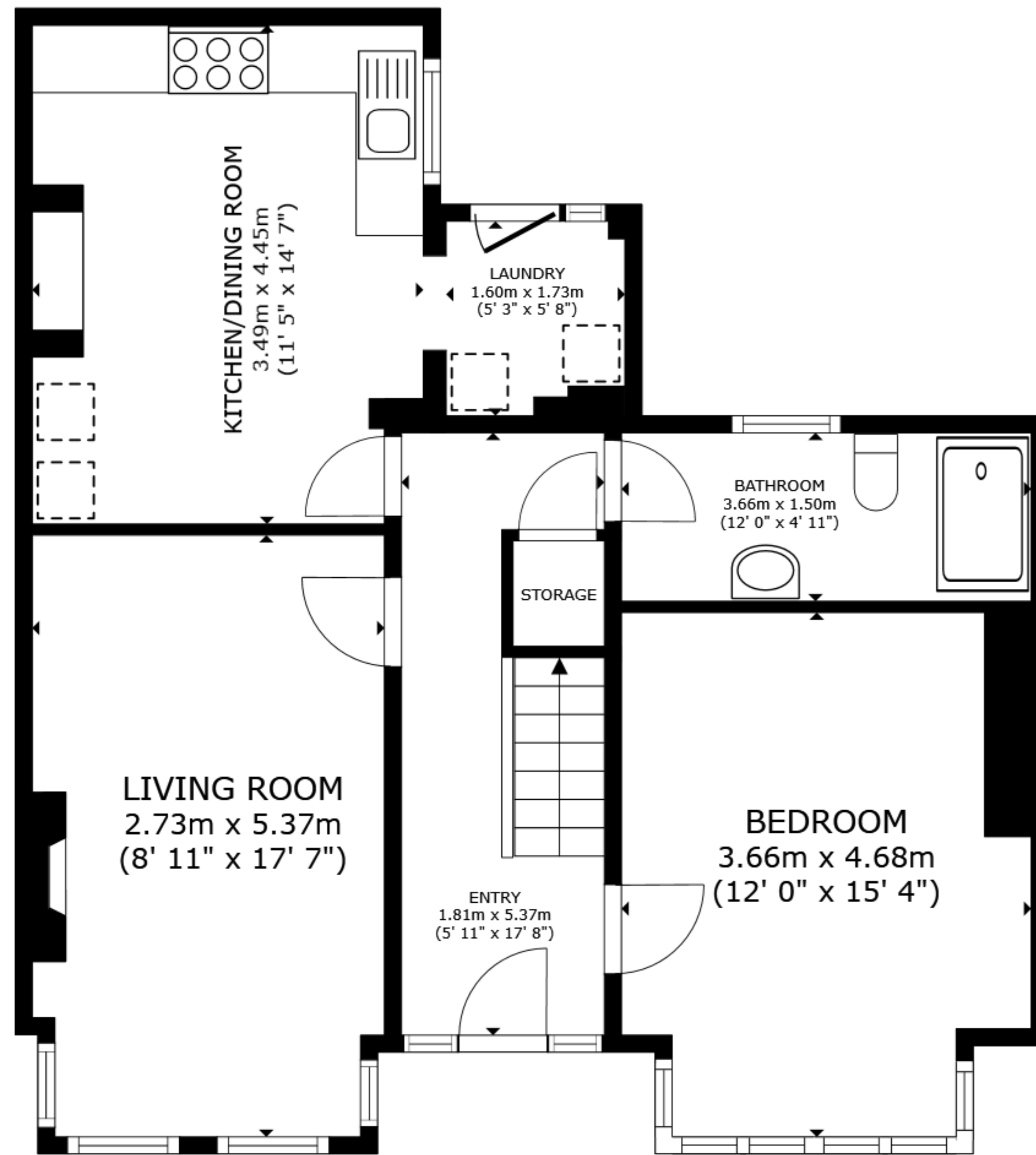
GROUND FLOOR
